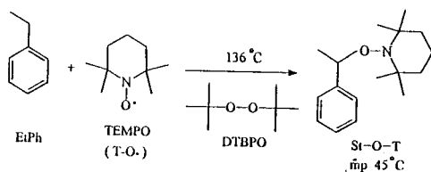
그림 4. Synthesis of a unimolecular initiator St-O-T from ethylbenzene and TEMPO in the presence of di- t -butyl peroxide (DTBPO).
