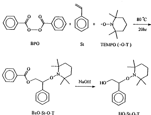
그림 3. Synthesis of a unimolecular initiator BzO-St-O-T from BPO and TEMPO in excess of St.
