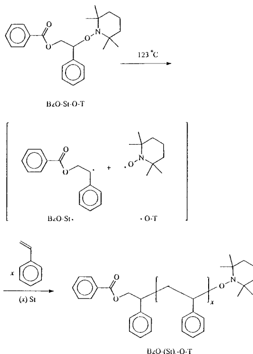
그림 2. Nitroxide-mediated 'living' free-radical polymerization of styrene using BPO/TEMPO as an initiation system.
