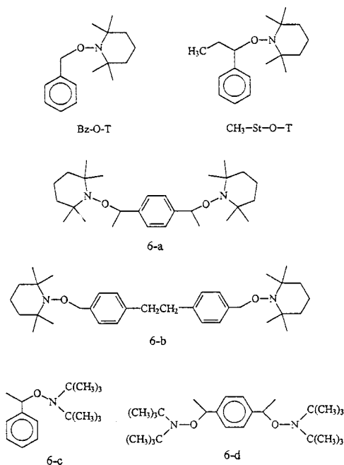
그림 6. Various nitroxide unimolecular initiators: a and b for bi-functional TEMPO, c and d for di- t -butyl nitroxide.
