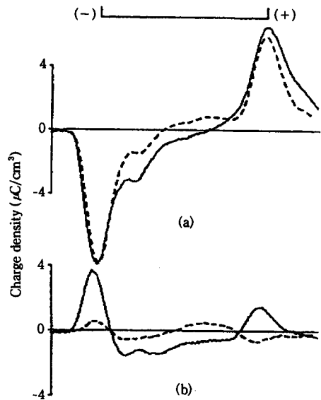
그림 14. Charge distributions in PE/ionomer blends(50/50 wt%): (a) During charging at 21.6 kV and (b) after discharging; PE/Surlyn 1601 blend (solid line), PE/Surlyn 1652 blend(dashed line). 35
