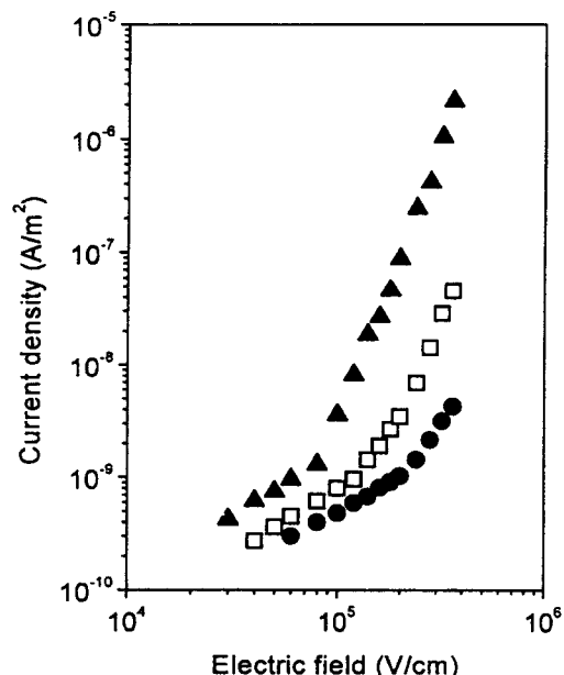
그림 12. Electrical conductive characteristic curves of PE-g-MAH (30 °C). LDPE ( \blacktriangle ), 0.05 wt% MAH ( \square ), 0.28 wt% MAH ( \bullet ). 33
