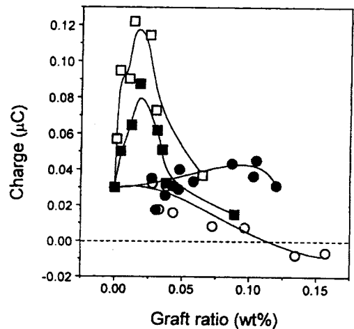
그림 19. Charge near the cathode of PE and acrylate grafted polyethylene immediately after short circuiting (40 kV/mm): PE-g-AA (○), PE-g-MA (□), PE-g-EA (■) and PE-g-nBA (●). 63
