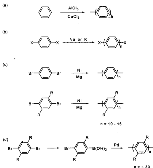
그림 1. Synthesis of poly( p -phenylene)s: (a) oxidative coupling, (b) reductive coupling by Na or K, (c) Yamamoto's route, and (d) Suzuki coupling using palladium catalyst.
