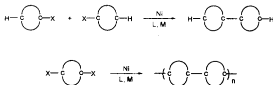
그림 5. Schematic diagram of coupling reaction with nickel catalyst.
