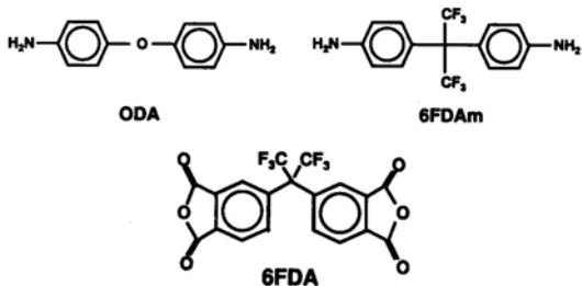
그림 4. Monomers lead to more flexible fluorinated polyimides.
