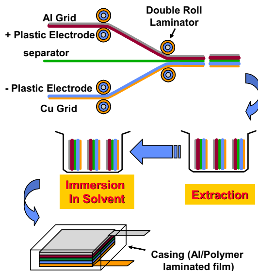
그림 6. Schematic diagram of battery manufacturing processes for Bellcore technology.
