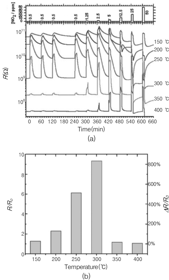
그림 8. (a) The resistance response during cyclic exposure to 10 min pulses with increasing concentrations of \text{NO}_2 mixed in dry air at various operating temperatures. (b) Sensitivity versus temperature histogram upon exposure to 500 ppb \text{NO}_2 in dry air. R_0 designates the baseline resistance in dry air.
