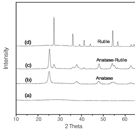
그림 11. XRD patterns of \text{TiO}_2 fibers heat-treated at different heat-treated temperature : (a) Untreated, (b) 250 °C 3 h, (c) 600 °C 3 h, and (d) 1,300 °C 3 h.
